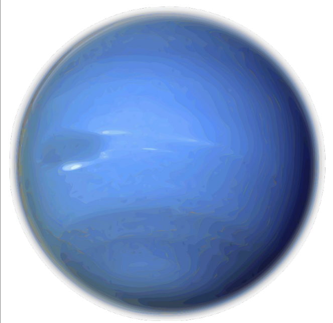
Neptune
