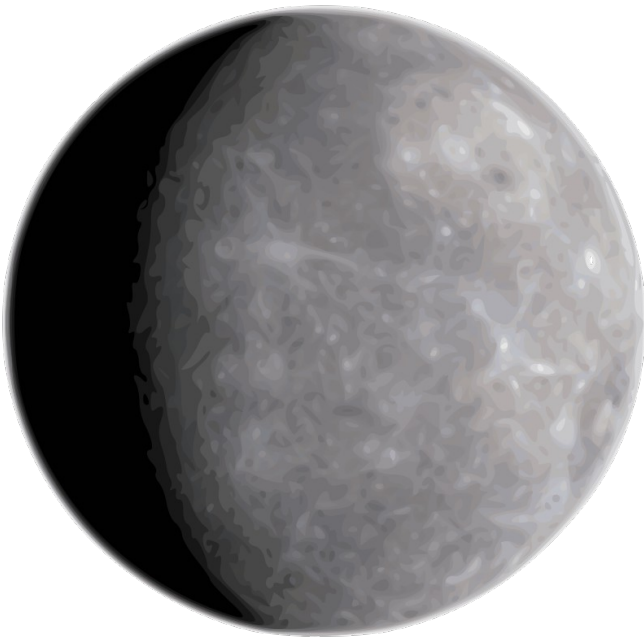
Mercury
