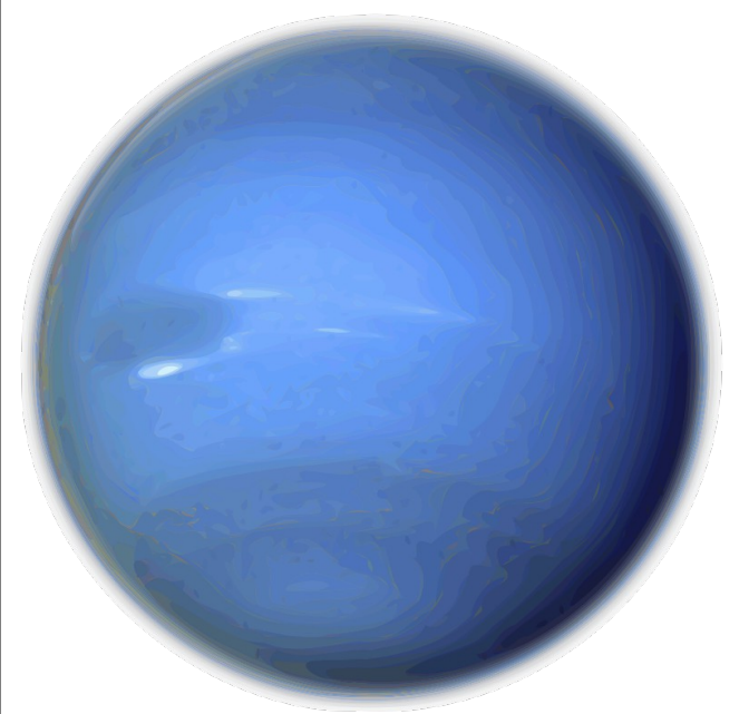
Neptune
